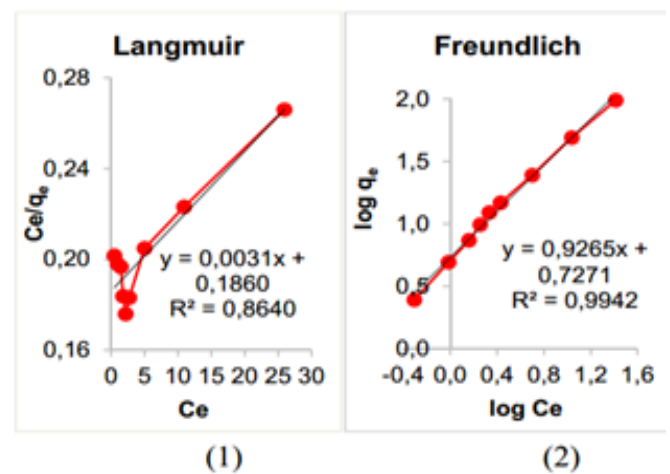
Gambar 5. Kurva Isoterm Adsorpsi Larutan Zat Warna Reactive Red Menggunakan AACB (1) Isoterm Langmuir (2) Isoterm Freundlich.
