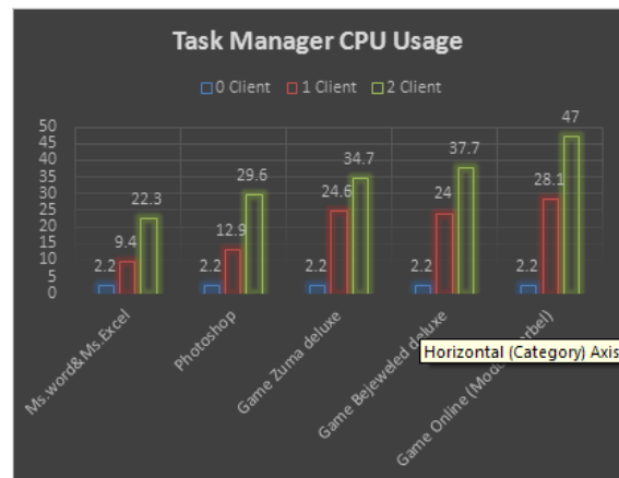
Gambar 4. CPU usage(tm)
