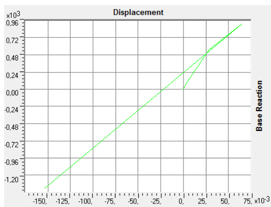
Gambar 5. Curve Capacity Push X (Data Pribadi Hasil Analisis SAP 2000, 2020)
