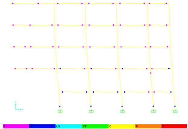
Gambar 3. 2D Sendi Plastis (SAP 2000 V.14, 2020)
