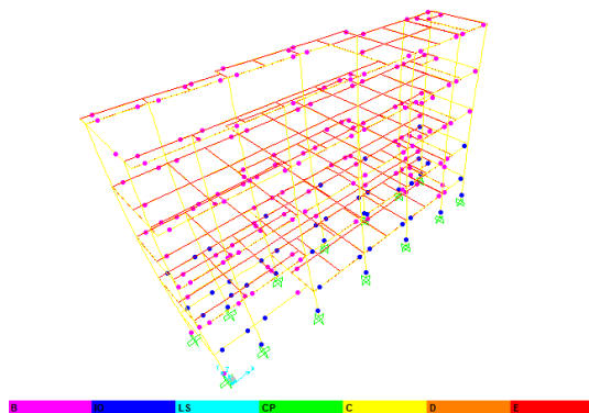
Gambar 8. 3D Sendei Plastis Push X Step 4 (Data Pribadi Hasil Analisis SAP 2000, 2020)
