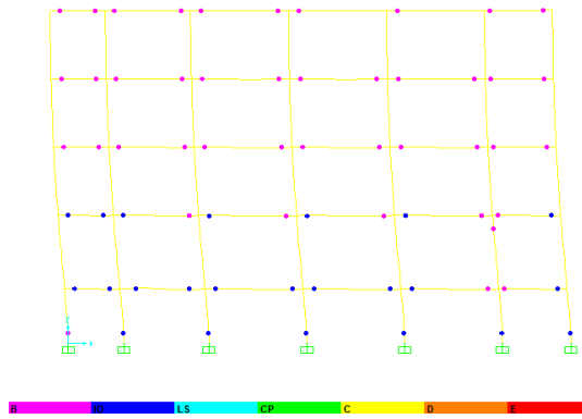
Gambar 7. 2D Sendei Plastis Push X Step 4 (Data Pribadi Hasil Analisis SAP 2000, 2020)
