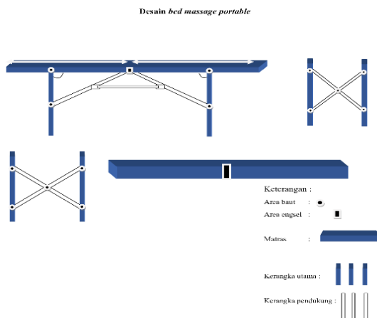
Figure 1. Desain Bed Massage Portable
