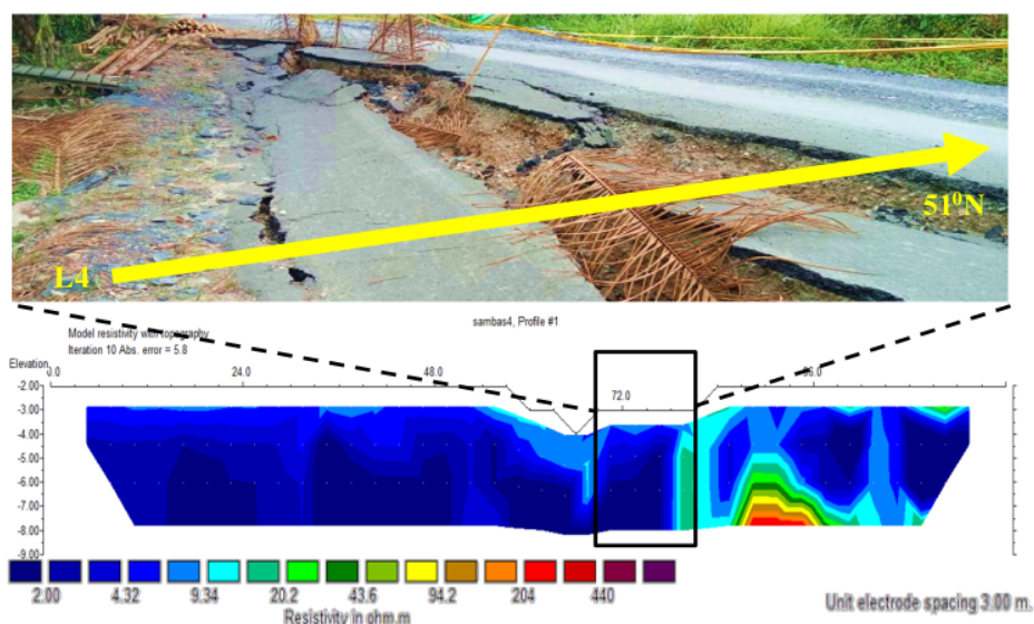
Gambar 8. Penampang inversi lintasan 4
