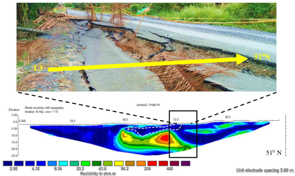
Gambar 7. Penampang inversi lintasan 3
