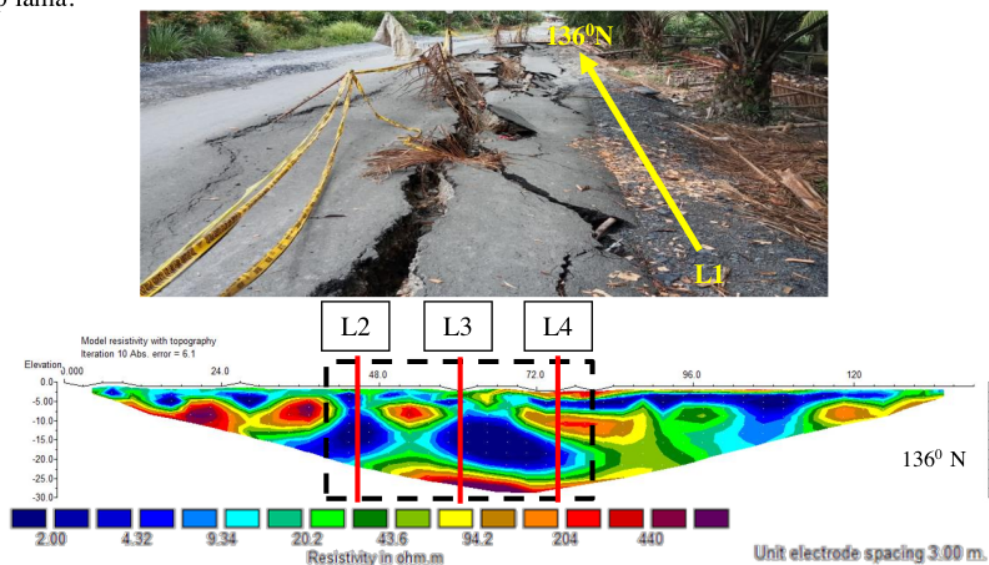
Gambar 5. Penampang hasil inversi lintasan 1
