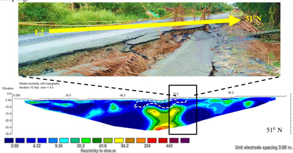
Gambar 6. Penampang inversi lintasan 2
