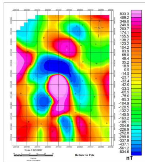
Figure 6. Reduce to Pole
