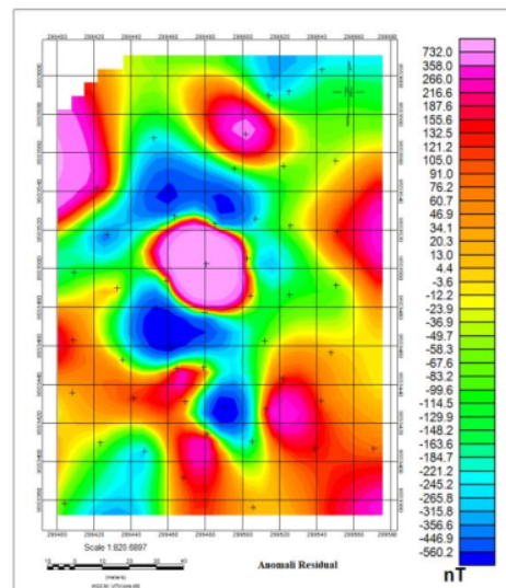
Figure 5. Residual Magnetic Anomaly
