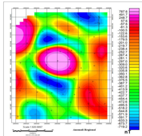
Figure 4. Regional Magnetic Anomaly
