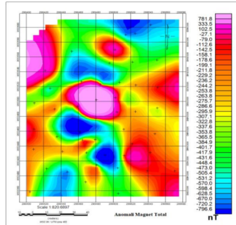
Figure 3. Total Magnetic anomaly
