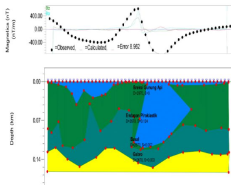
Figure 9. Model slice B-B' from Slice Map Reduction to Pole
