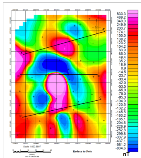
Figure 7. Determination Slice Anomaly on the Reduction to Pole
