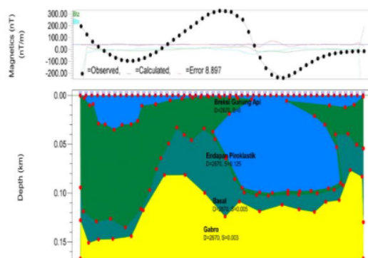
Figure 8. Model slice A-A' from Slice Map Reduction to Pole
