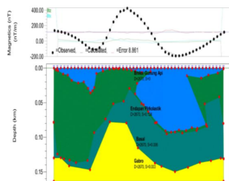
Figure 10. Model slice C-C' from Slice Map Reduction to Pole
