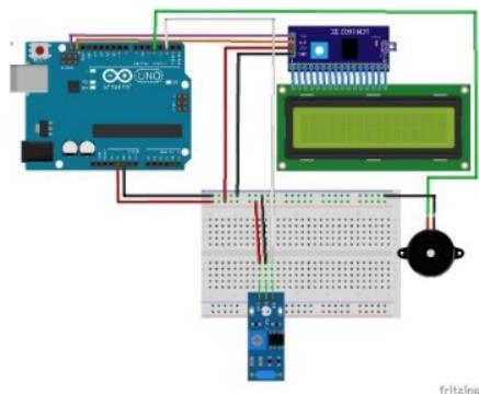
Figure 3. Electronic schematic
