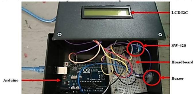
Figure 7. Electronic system
