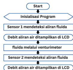
Gambar 4. Diagram Sistem Alat Peraga
