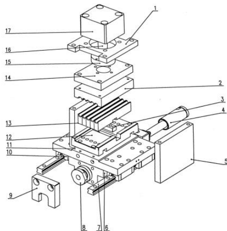
(Bending Mechanism)
